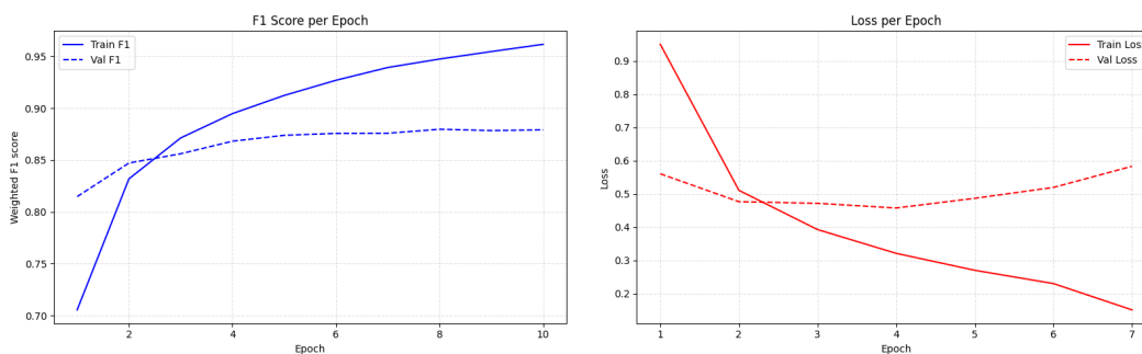
Figure 8. Training the text model, weighted-F1 (left) and cross-entropy loss (right) per epoch. The two panels disagree on when to stop, and that disagreement is the point. Validation loss reaches its minimum at about epoch four and then rises steadily, while validation F1 continues to improve to roughly 0.880 at about epoch eight. The model is becoming more confident on the cases it still gets wrong, which cross-entropy punishes because it scores confidence, while the arg-max decision that F1 measures keeps improving. Selecting on validation loss therefore stops around epoch four and costs about one point of weighted-F1 (0.87 against 0.88) on a task whose official metric is weighted-F1. Validation F1 is already 0.815 after a single epoch, above the challenge text baseline of 0.8113.
