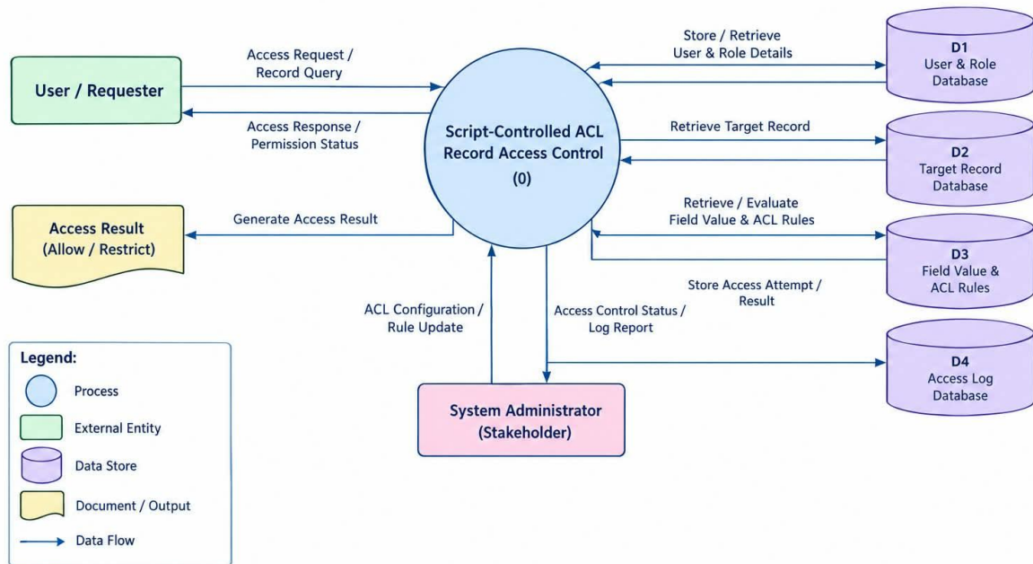
Data Flow Diagram: Script-Controlled ACL – Restrict Record Access Based on Field Value
