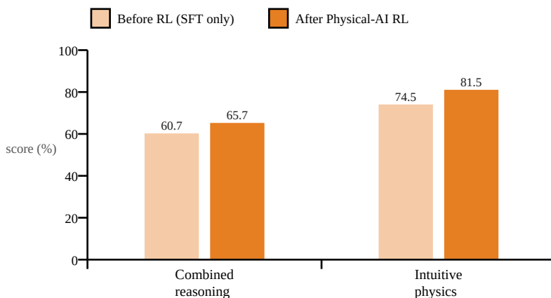
Figure 14. Adding the GRPO reinforcement-learning stage raised the 7B model by +5.0 points (combined reasoning) and +7.0 points (intuitive physics) — evidence that post-training, not just size, drives physical reasoning. Source note: research-page figures; arXiv v1 reports different magnitudes (e.g. intuitive physics 65.7→68.7). The direction — RL helps — is consistent across both.
