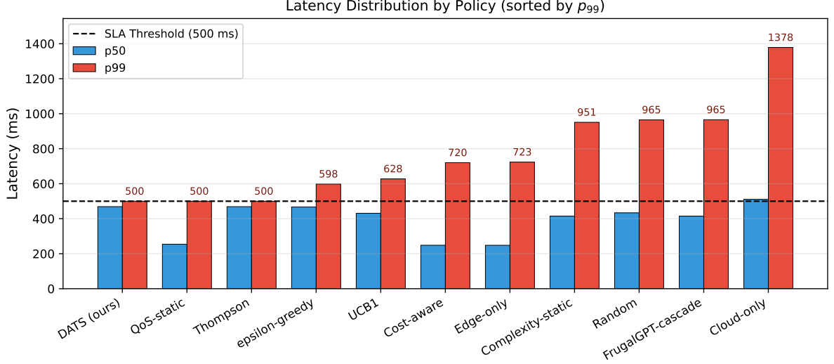
Figure 3: Latency distribution by policy, sorted by p_{99} . DATS, QoS-static, and Thompson Sampling keep p_{99} at the 500 ms SLA threshold; \epsilon -greedy and UCB1 trail by \sim 100 – 130 ms; all non-learning baselines miss the threshold by 200 ms or more.
