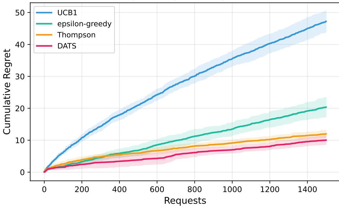
Adaptation Speed Comparison
