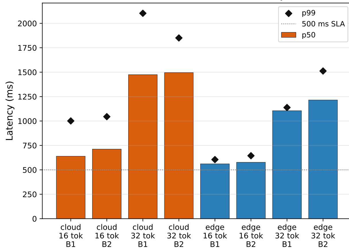
Measured RTX 5090 Inference Latency
