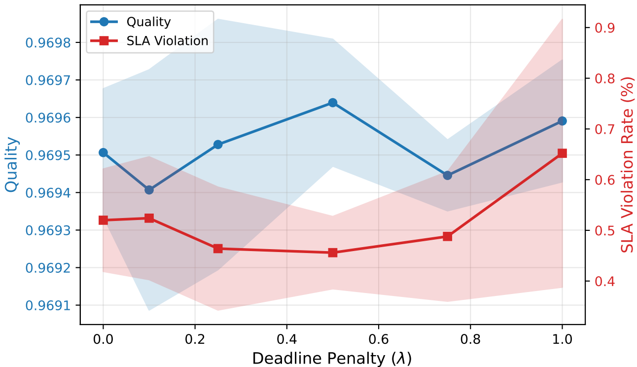
Effect of Deadline Penalty \lambda (shaded: \pm 1\sigma across seeds)
