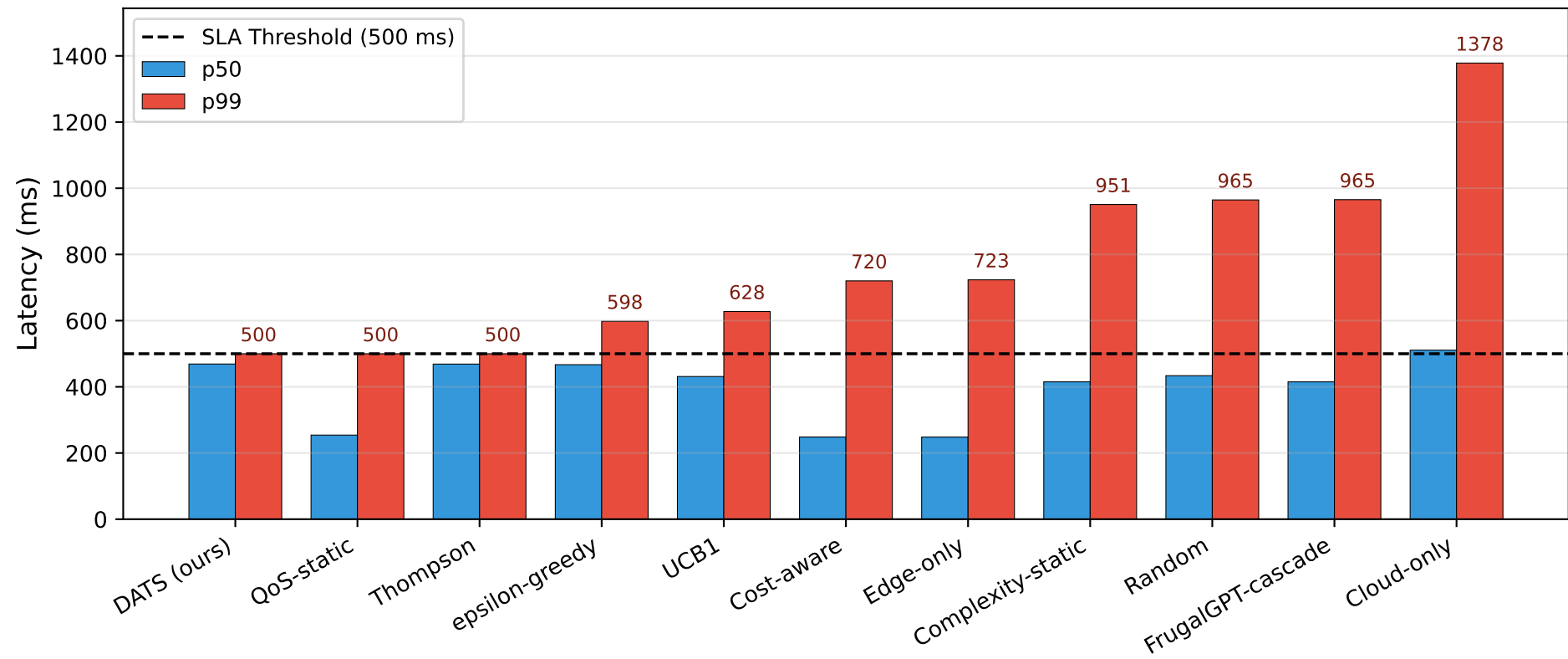
Latency Distribution by Policy (sorted by p_{99} )
