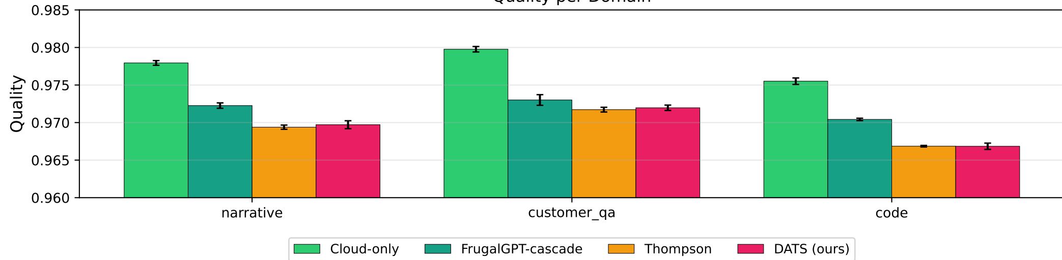
Quality per Domain
