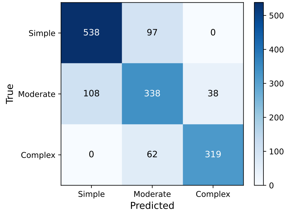
Confusion Matrix (acc=0.80)
