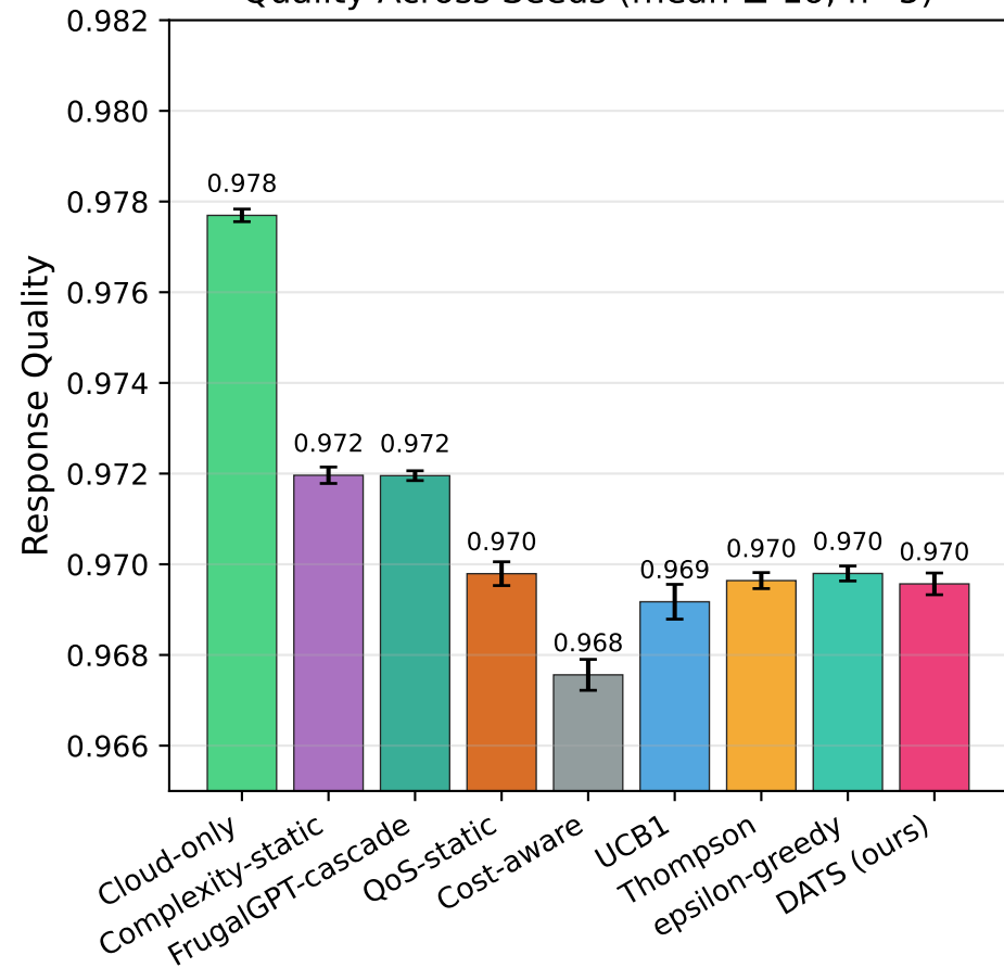
Quality Across Seeds (mean \pm 1\sigma , n=5)
