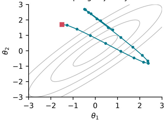
leapfrog trajectory
