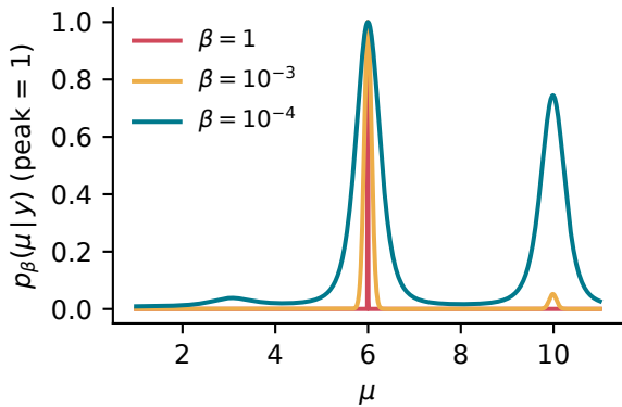
tempered posteriors
