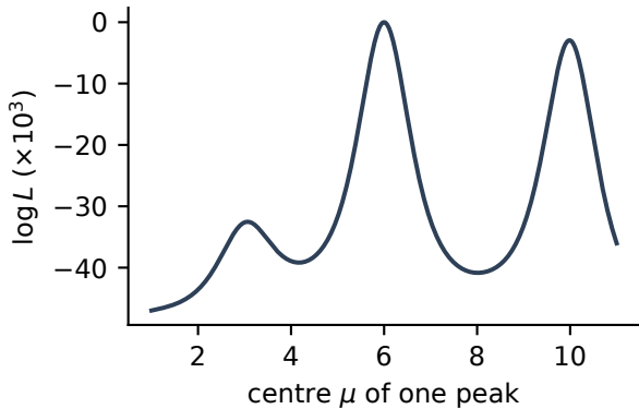
likelihood: many local optima
