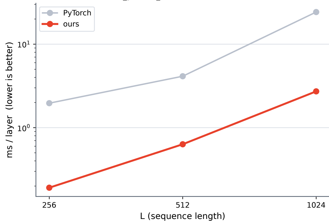
Bidirectional trimul forward (B=1, bf16, d_pair=d_hidden=128 → back over 256ch)
