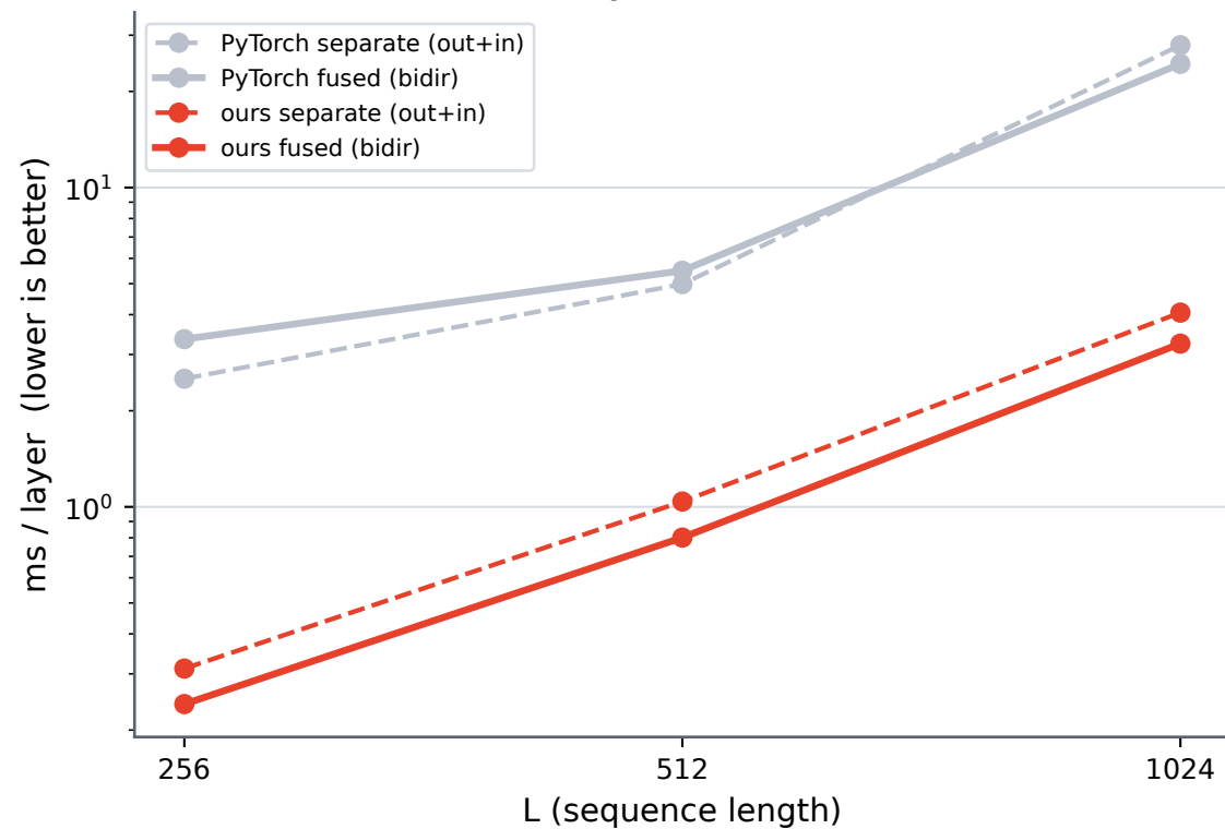
Fused vs separate trimul directions (B=1, bf16, per-direction h=128)
