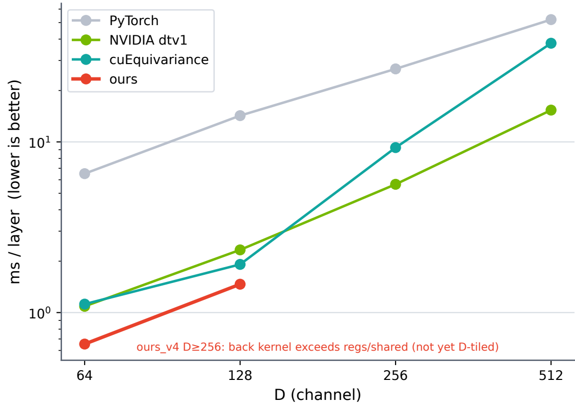
trimul forward, L=1024 (B=1, bf16, no mask)
