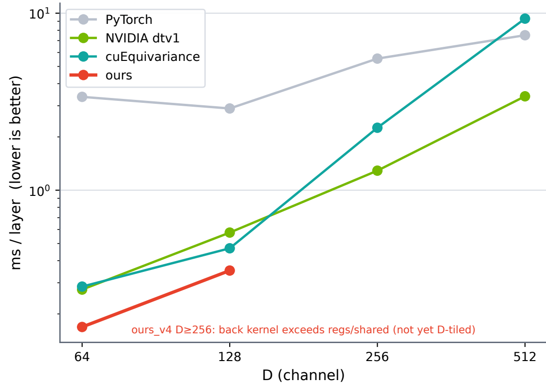
trimul forward, L=512 (B=1, bf16, no mask)
