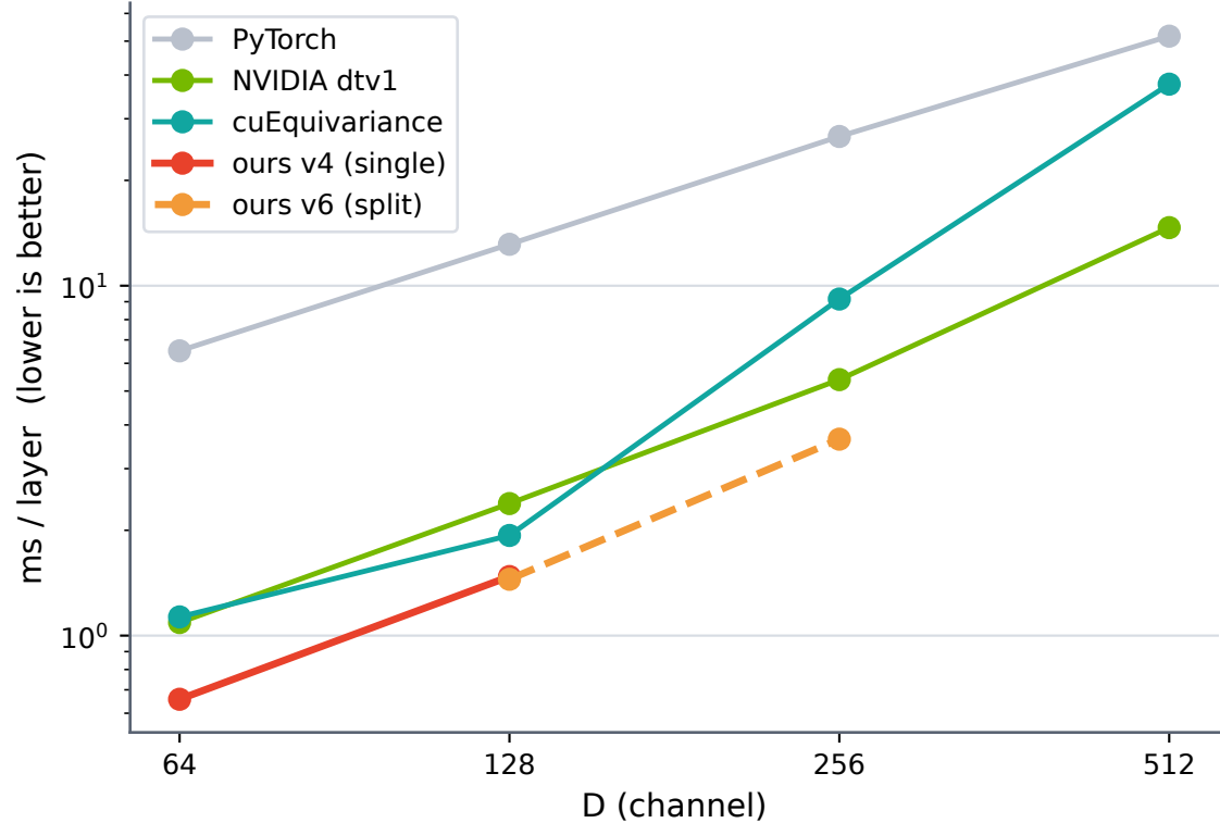
trimul forward, L=1024 (B=1, bf16, no mask) v4=single fused back, v6=split (cute LNLinear + triton GateElem)
