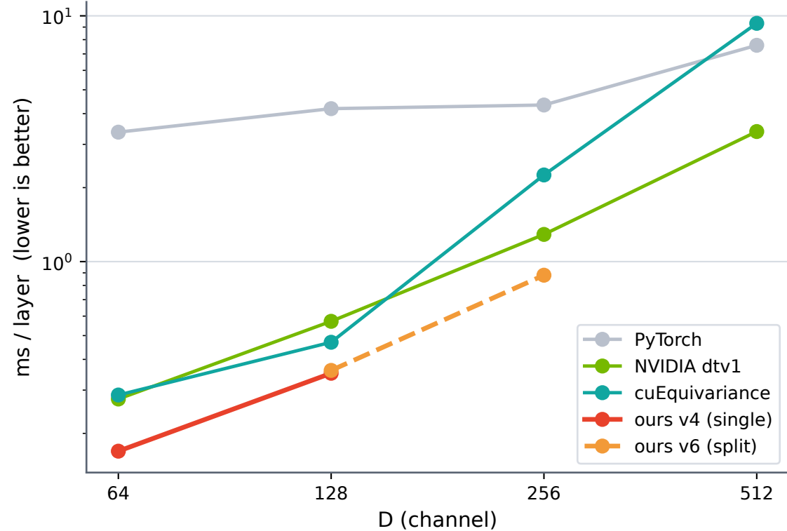
trimul forward, L=512 (B=1, bf16, no mask) v4=single fused back, v6=split (cute LNLinear + triton GateElem)
