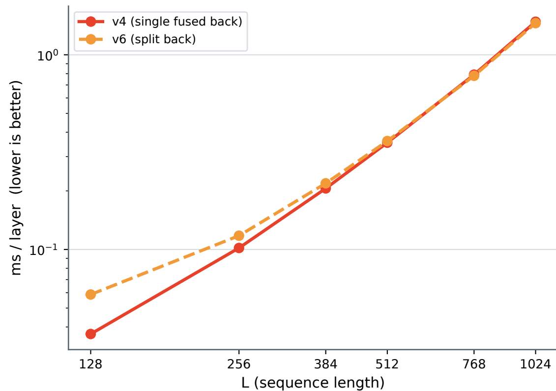
v4 vs v6 back, D=128 (B=1, bf16)
