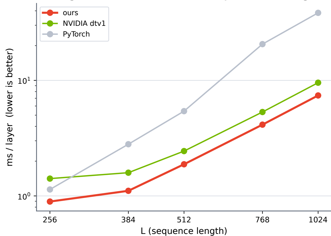
Single-dir trimul fwd+bwd (torch.compile, exact training)
