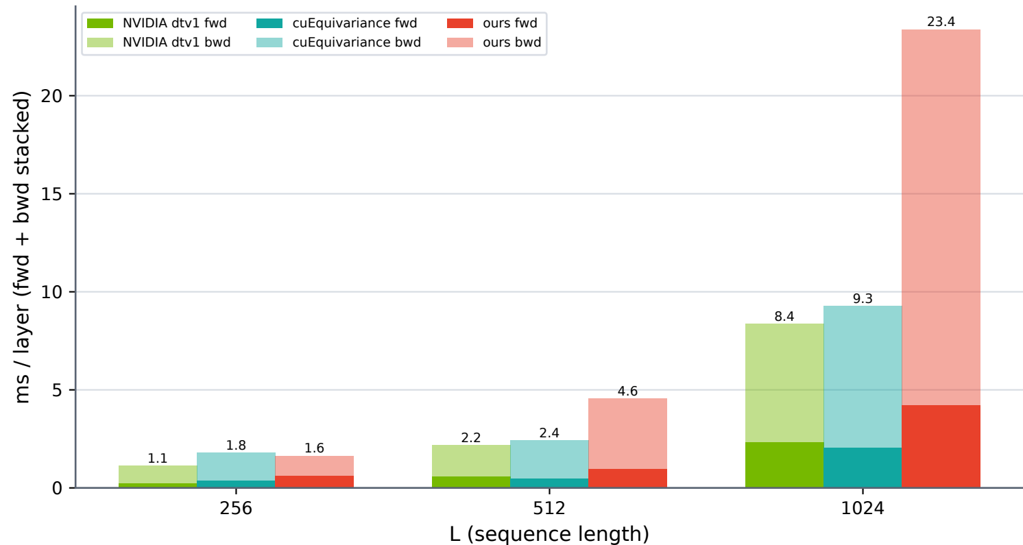
Single-dir trimul fwd+bwd (EAGER): ours_v6 vs dtv1 / cuEquiv (pytorch omitted ~4x; backward is where v6 loses)
