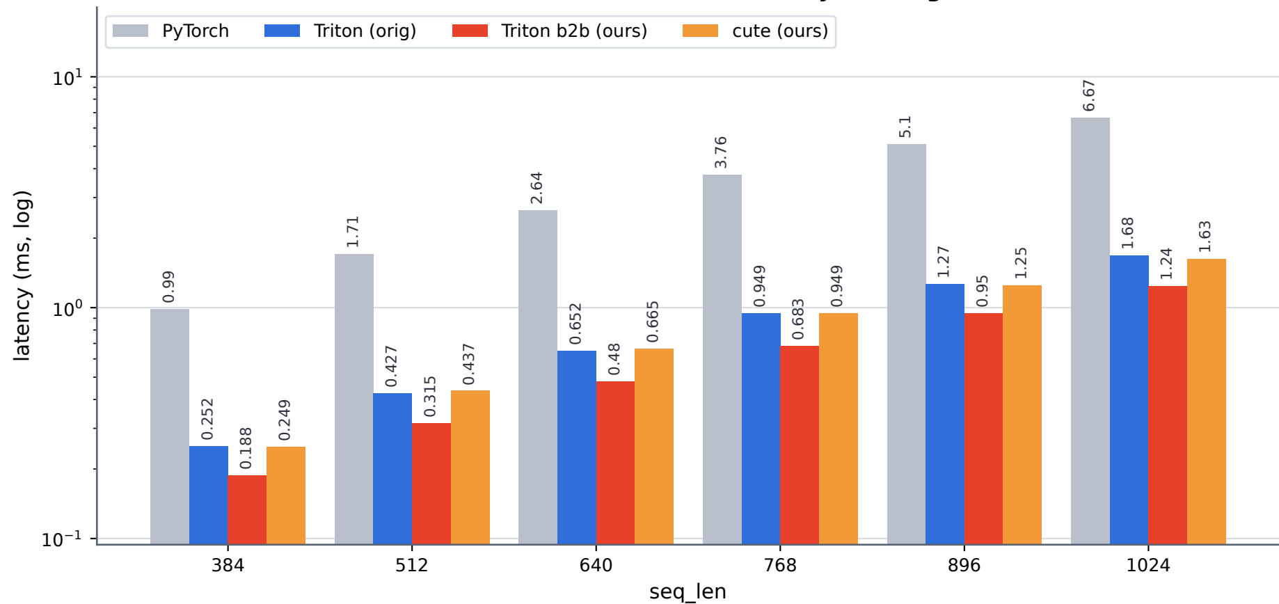
Transition forward (H100 bf16, d=128, n=4) — latency (ms, log scale; lower is better)
