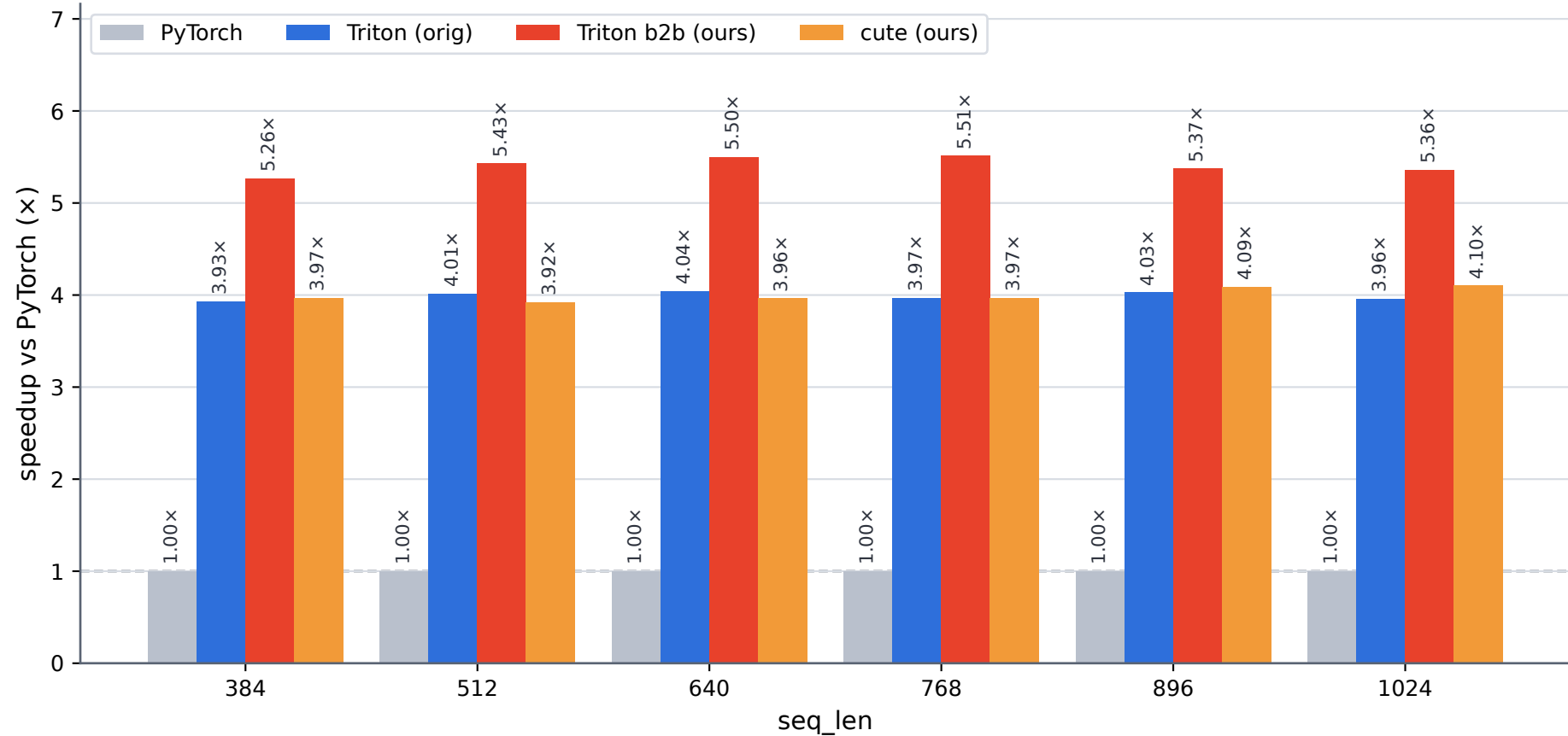
Transition forward (H100 bf16, d=128, n=4) — speedup vs PyTorch default (higher is better)
