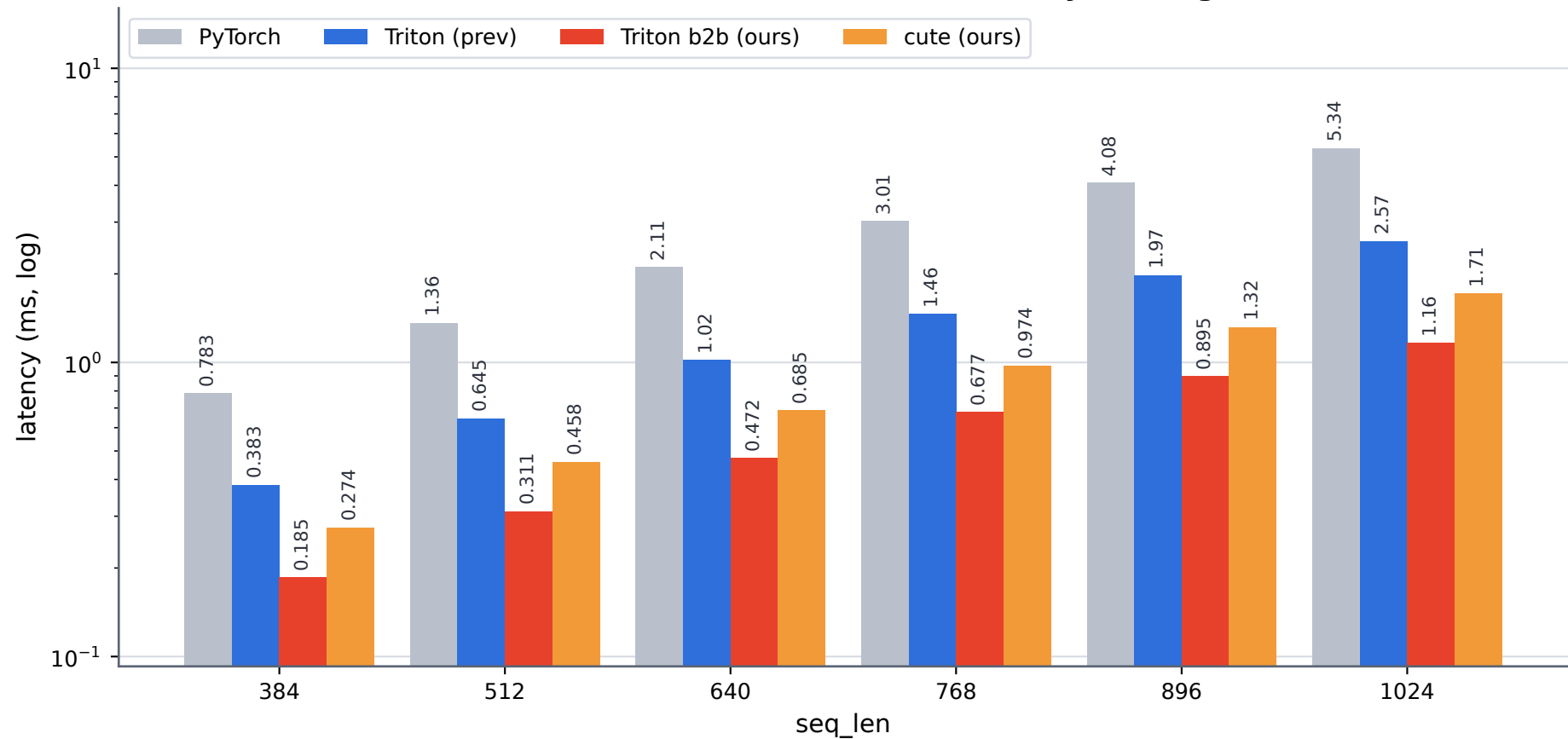
Transition module forward (H100 bf16, d=128, n=4) — latency (ms, log scale; lower is better)
