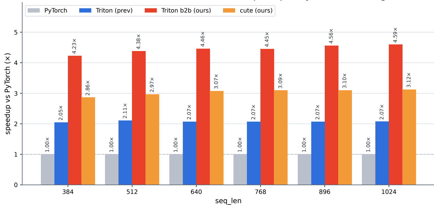
Transition module forward (H100 bf16, d=128, n=4) — speedup vs PyTorch default (higher is better)
