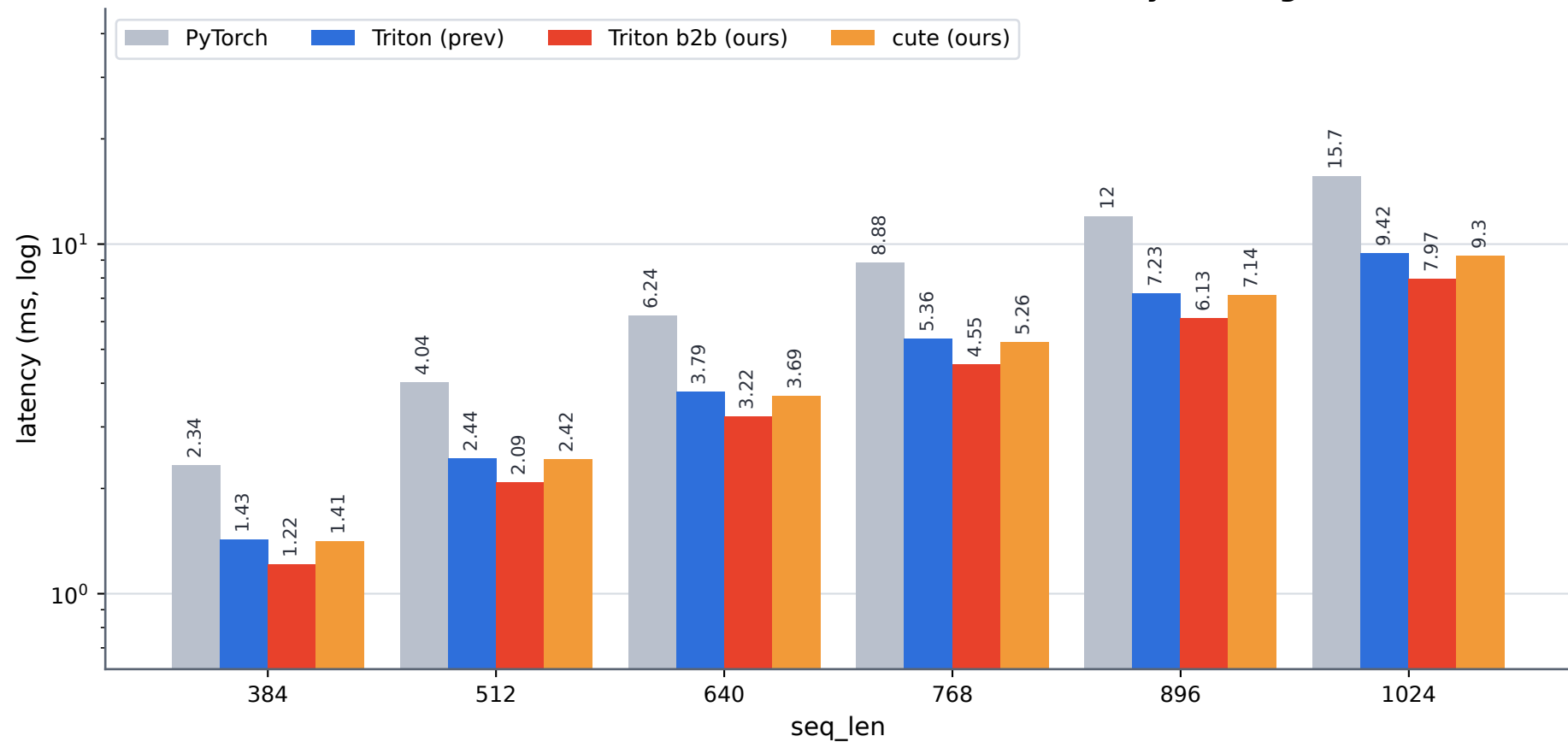
Transition module forward+backward (H100 bf16, d=128, n=4) — latency (ms, log scale; lower is better)
