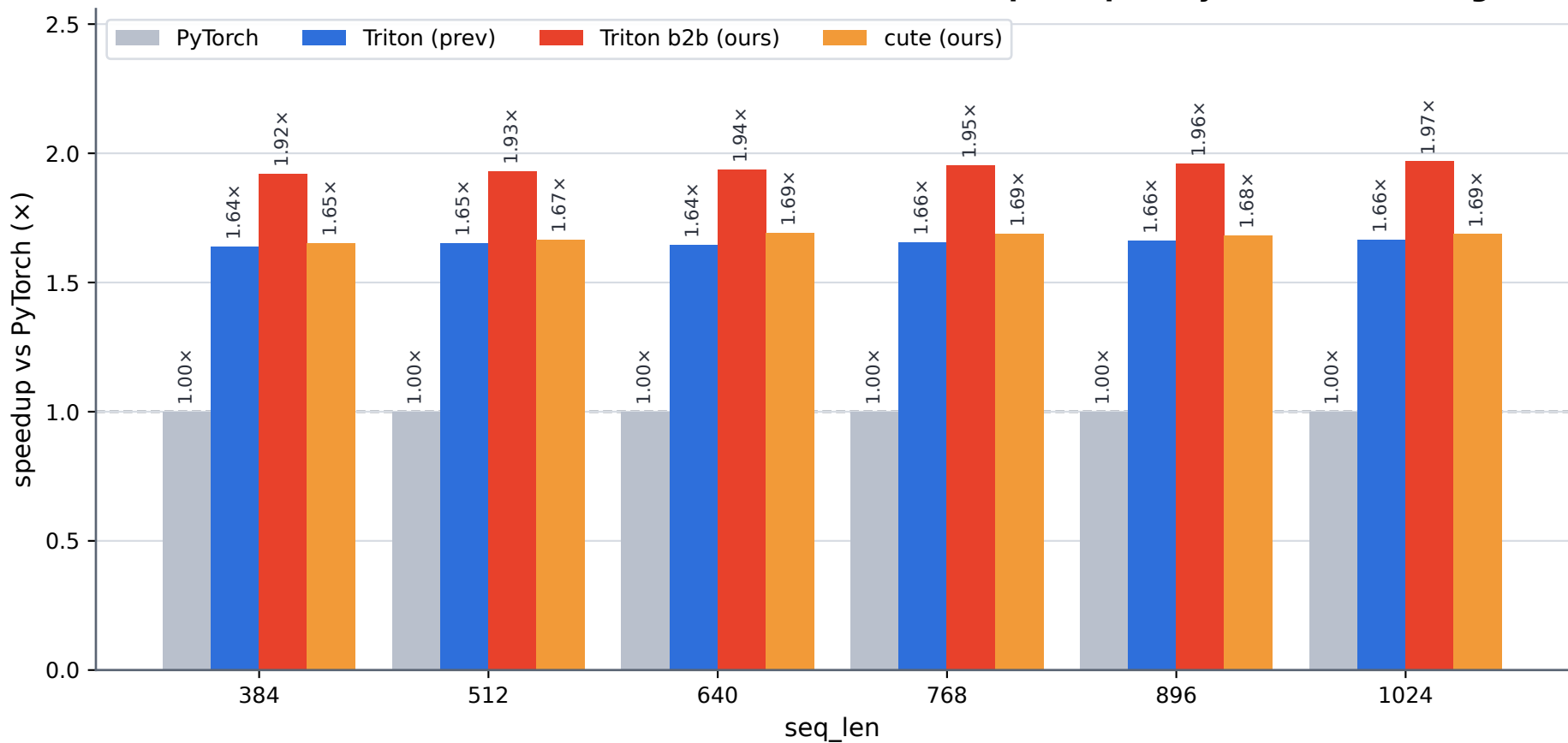
Transition module forward+backward (H100 bf16, d=128, n=4) — speedup vs PyTorch default (higher is better)
