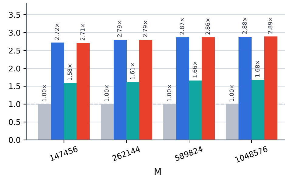
d = 384
