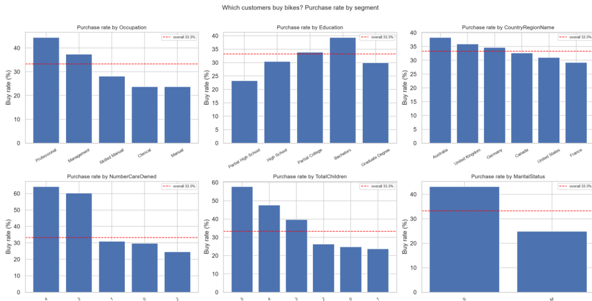
Figure 2: Purchase rate by segment against the overall base rate. Household and occupation attributes separate more strongly than geography.
