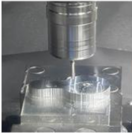
Intermediate Machining Stage
