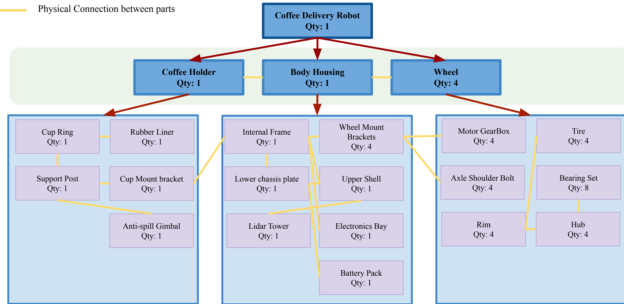
Part Hierarchy
