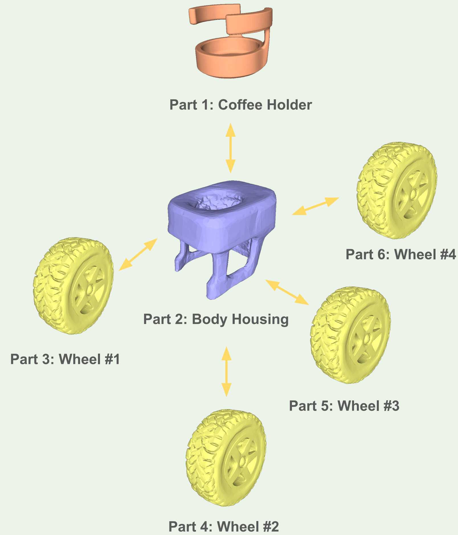
Top Level Assembly Structure
