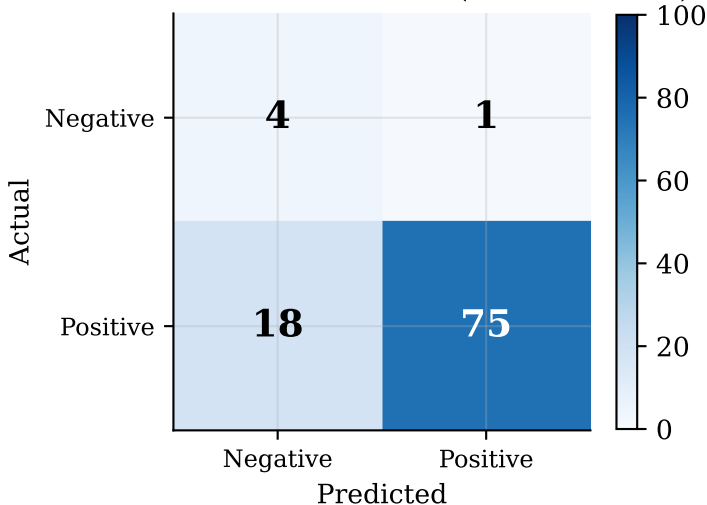
Confusion Matrix — ADULT (Influence Func.)
