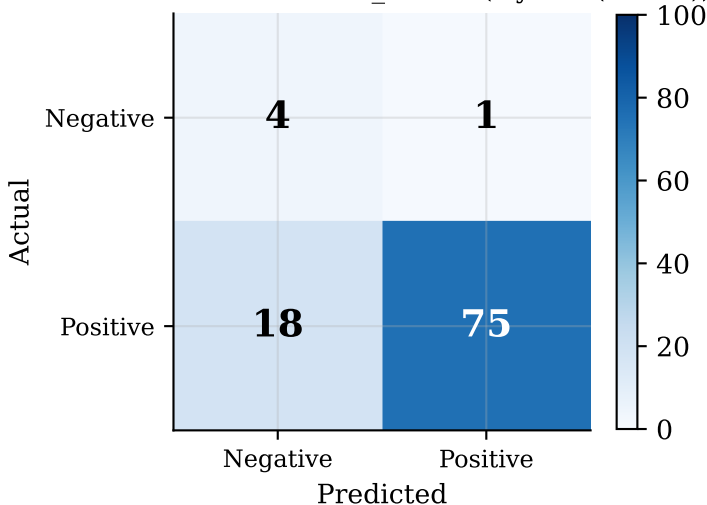
Confusion Matrix — AG_NEWS (Hybrid (HAUC))
