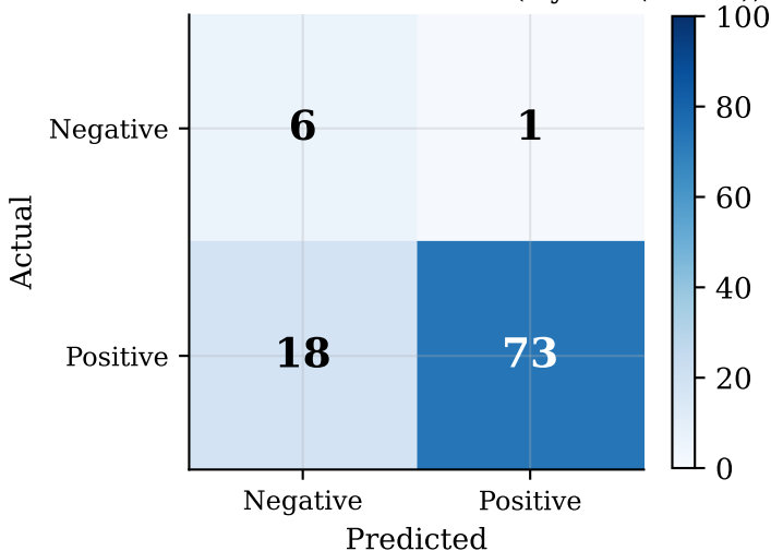
Confusion Matrix — CIFAR10 (Hybrid (HAUC))
