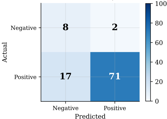
Confusion Matrix — CIFAR10 (Influence Func.)
