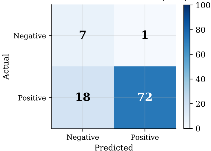
Confusion Matrix — CIFAR10 (SISA)
