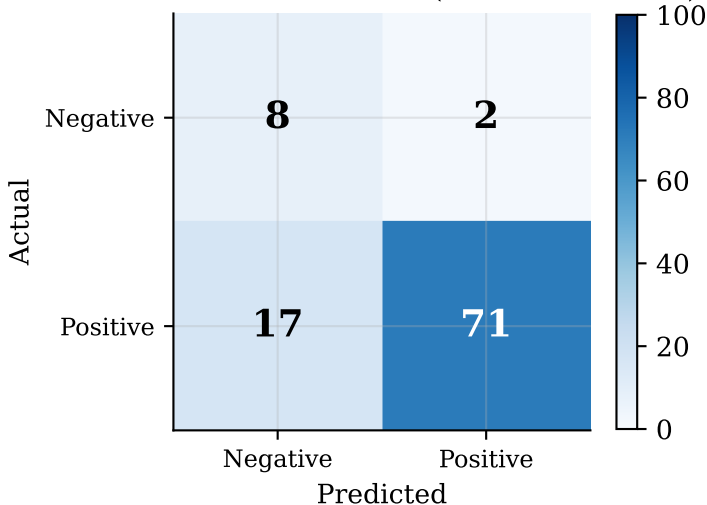
Confusion Matrix — IMDB (Certified Removal)
