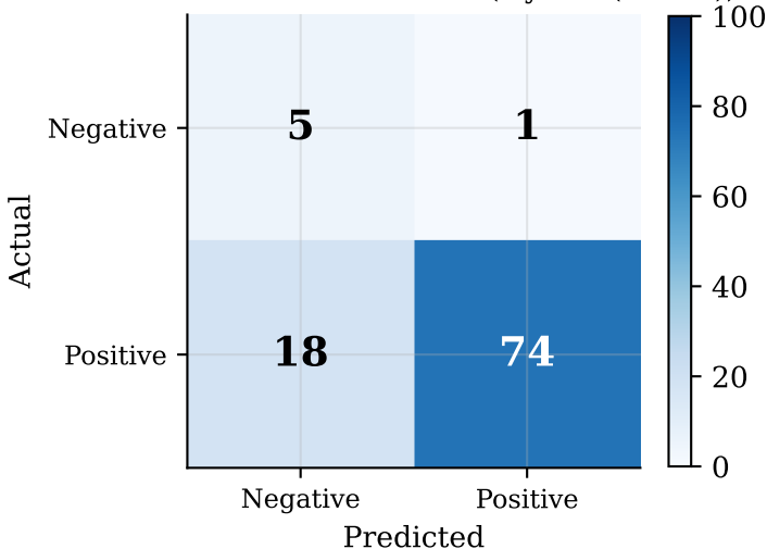
Confusion Matrix — IMDB (Hybrid (HAUC))
