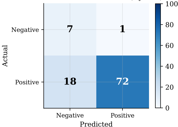
Confusion Matrix — PURCHASE100 (Hybrid (HAUC))
