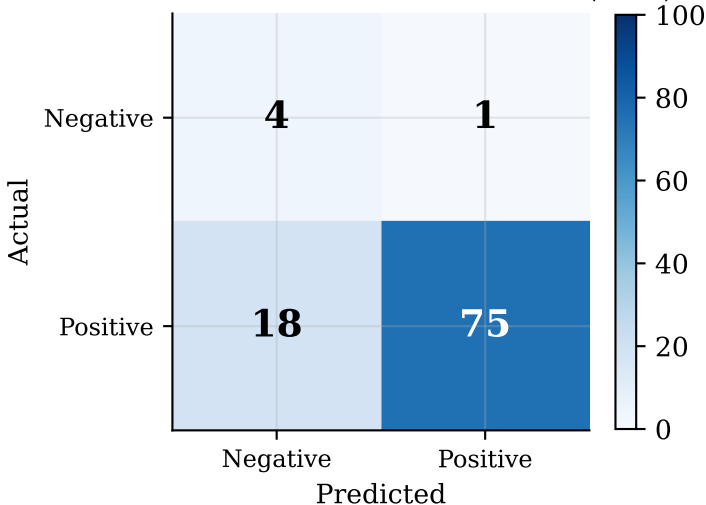
Confusion Matrix — PURCHASE100 (SISA)
