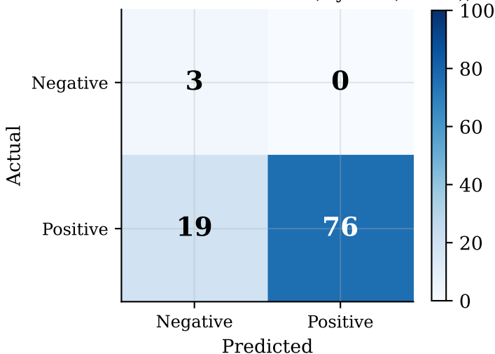
Confusion Matrix — SST2 (Hybrid (HAUC))
