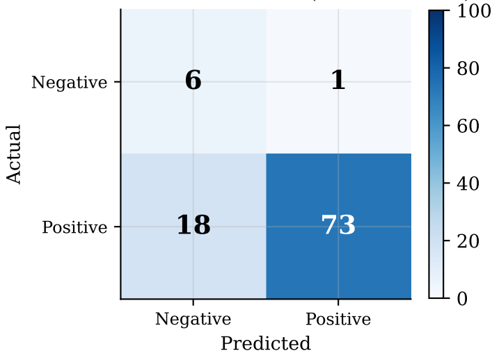
Confusion Matrix — SST2 (Influence Func.)
