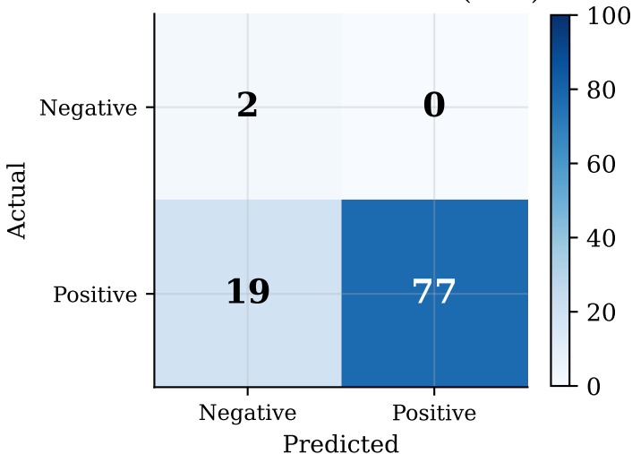
Confusion Matrix — SST2 (SISA)
