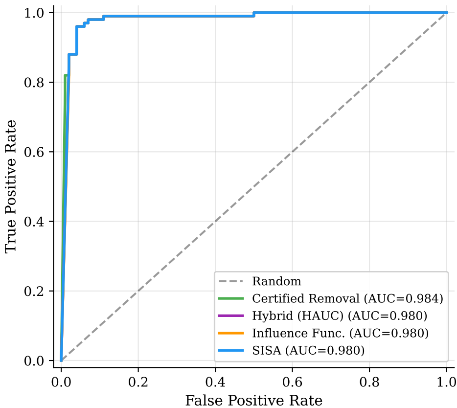
ROC Curves — ADULT
