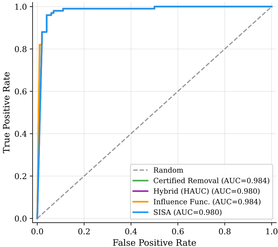
ROC Curves — AG_NEWS
