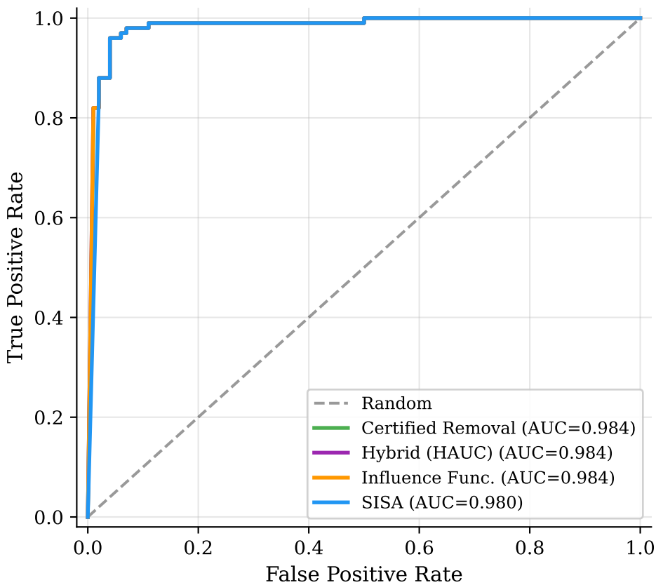
ROC Curves — IMDB
