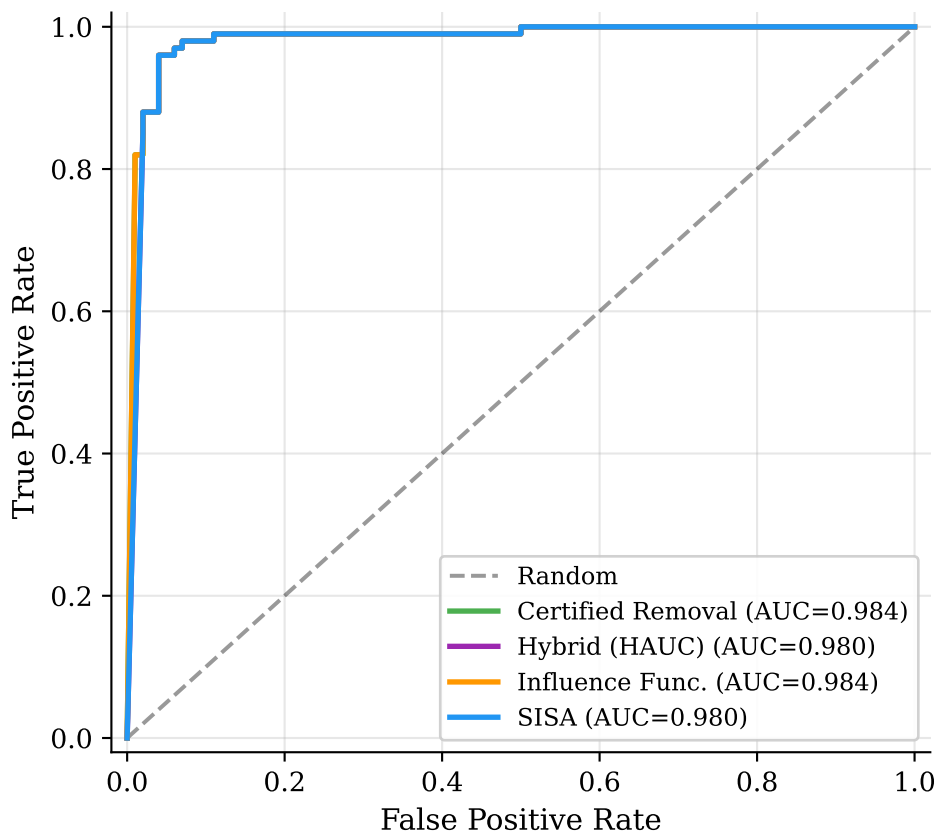
ROC Curves — SST2
