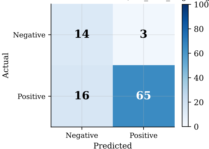
Confusion Matrix — MNIST (fine_tune_forgetting)
