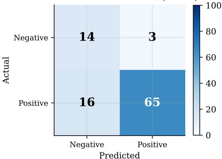
Confusion Matrix — MNIST (retrain)
