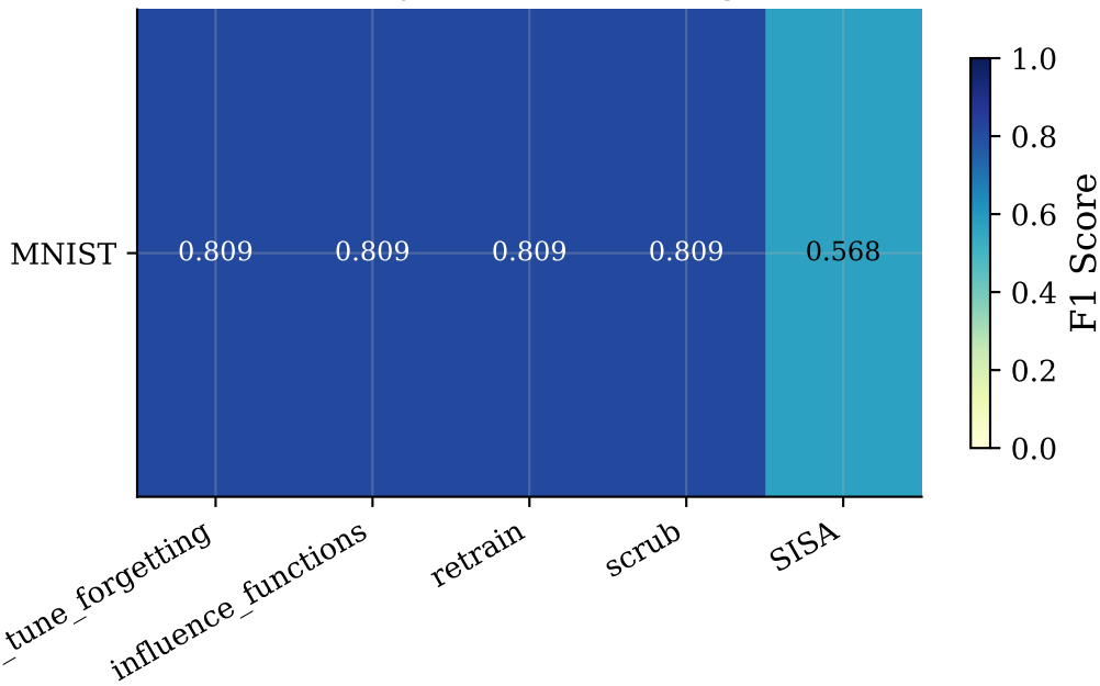
F1 Score by Dataset and Algorithm
