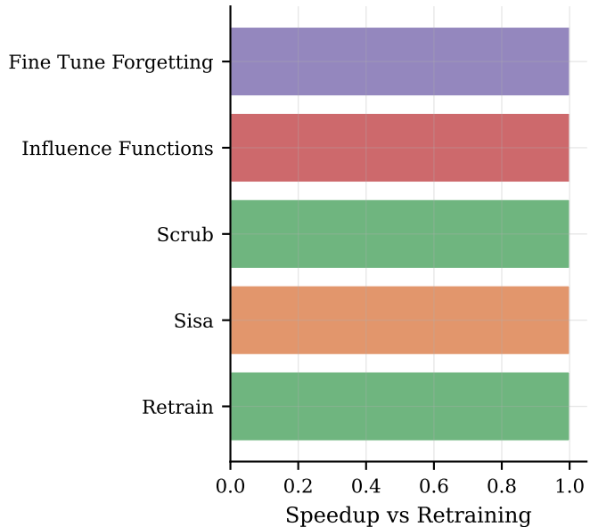
Speedup Factor
